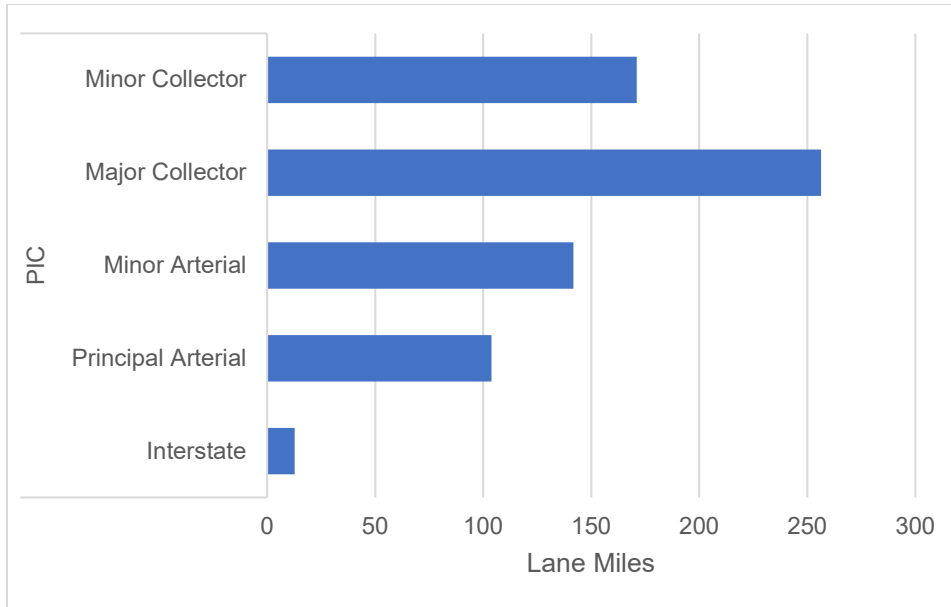
Figure K. 25 Pickaway County Sum of Lane Miles by Functional Classification, 2023
